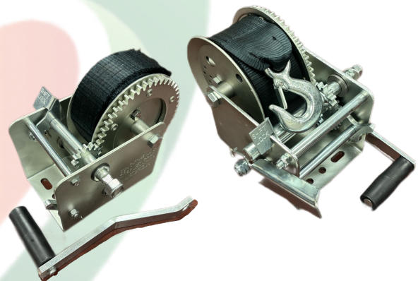
Two-Speed Winches in Zinc Plated Finish from 2,600 to 3,700lb Capacity (3,200 & 3,700lb have brake)
