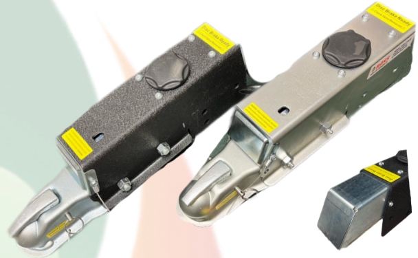
Drum & Disc Brake Actuator, 6,600lb Capacity in Black and Zinc Plated finishes. Rear cover available
